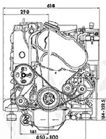
Frontal view
